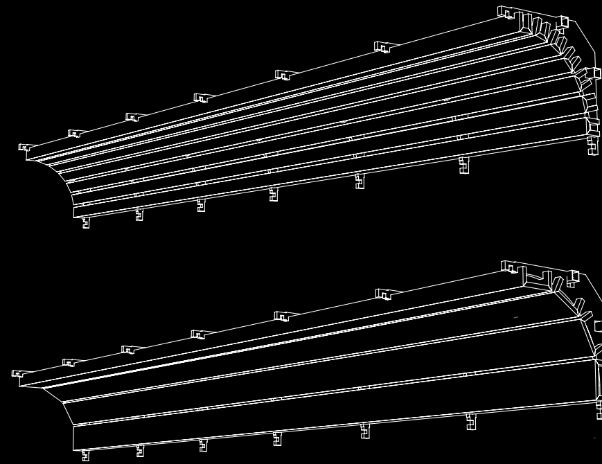
LANDSCAPE TRANSITION NARROW SET 108" 2745mm w x 11.67" 296mm h
